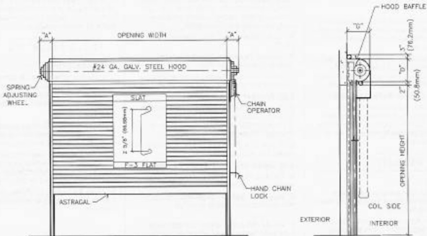
COIL SIDE ELEVATION RIGHT HAND OPERATION AS SHOWN LEFT HAND OPERATION IS OPPOSITE AS SHOWN
